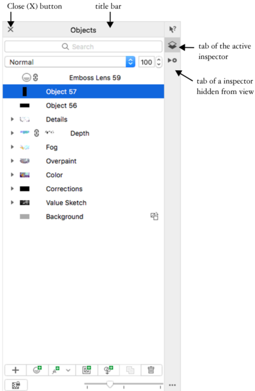
An example of an inspector is the Objects inspector. The Objects inspector displays thumbnails of the image background and each object layer, as well as command buttons and options related to objects.
